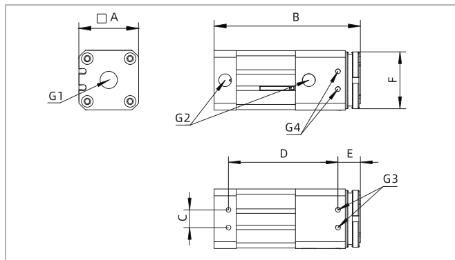
SLG-H High temperature resistance
