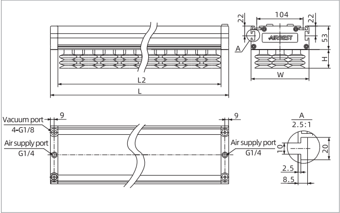
TXC130×1000/1200/1400-B Suction cup type
